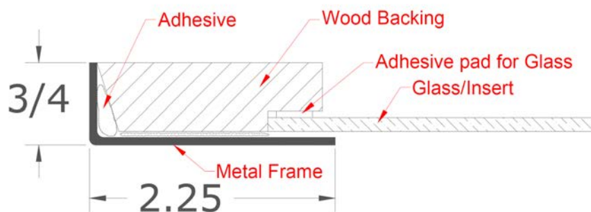
Assembly Detail
