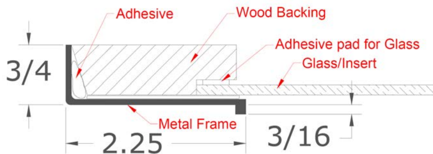
Assembly Detail
