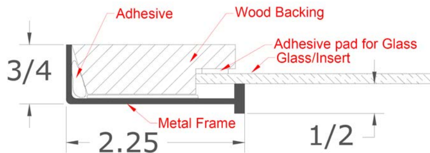
Assembly Detail
