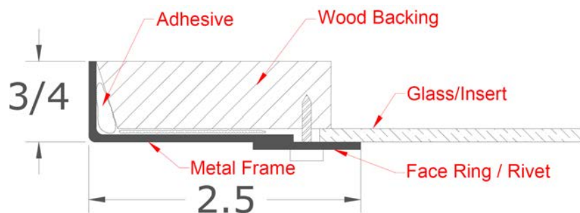
Assembly Detail
