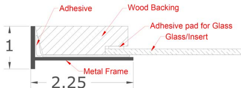
Assembly Detail
