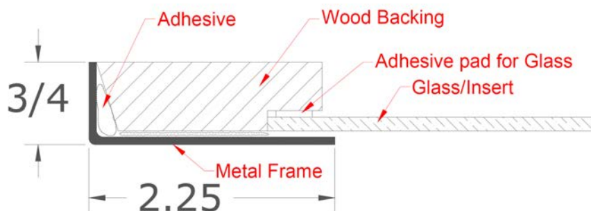
Assembly Detail
